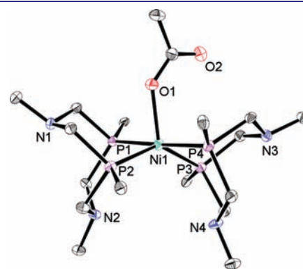
Figure 2. Perspective thermal ellipsoid plot of the crystal structure of [\text{Ni}(\text{P}^{\text{Ph}}_2\text{N}^{\text{Bn}}_2)_2(\text{OAc})](\text{BF}_4) . Thermal ellipsoids are shown at the 50% probability level. The Ni1–O1 distance is 2.09 Å, whereas Ni1–O2 is 3.56 Å. For clarity, hydrogen atoms and uncoordinated counterions are omitted, and only the first carbon of the nitrogen and phosphorus substituents is shown.
