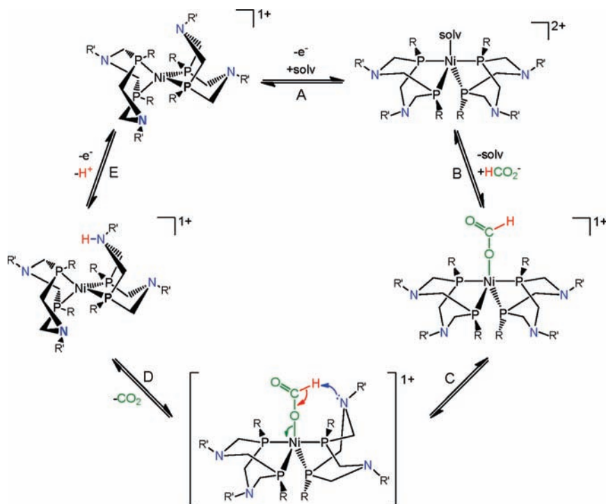
Scheme 2. Proposed Reaction Scheme for Electrocatalytic Formate Oxidation
