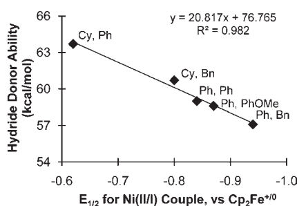
Figure 5. Correlation of the potential of the Ni(II/I) couple for [\text{Ni}(\text{P}^{\text{R}}_2\text{N}^{\text{R}'})_2(\text{CH}_3\text{CN})]^{2+} complexes with the hydride donor ability for the corresponding hydrides. The designations for each point (R, R') indicate phosphorus and nitrogen substituents, respectively.
