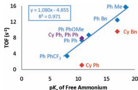
Figure 10. Correlation of TOF for electrocatalytic formate oxidation with the \text{p}K_{\text{a}} of the free primary ammonium ( \text{R}'\text{NH}_3^+ ) used to synthesize the corresponding \text{P}^{\text{R}}_2\text{N}^{\text{R}'} ligands for each \text{Ni}(\text{P}^{\text{R}}_2\text{N}^{\text{R}'})_2\text{-(CH}_3\text{CN)}_2^{2+} complex. The data point labels in the figure refer to the R and R' substituents, respectively, and the trend line and corresponding equation are only for R = Ph.
